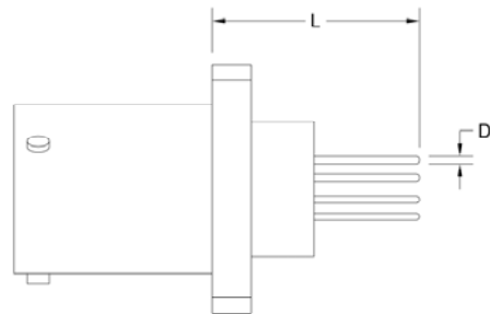
SQUARE FLANGE MOUNTING
