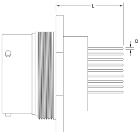
JAM-NUT MOUNTING
